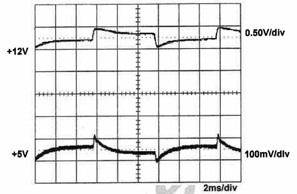
+12Vsb step from 0.67A to 3.33A other output at 60% load
