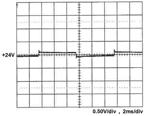
+24V step from 2.33A to 11.66A
