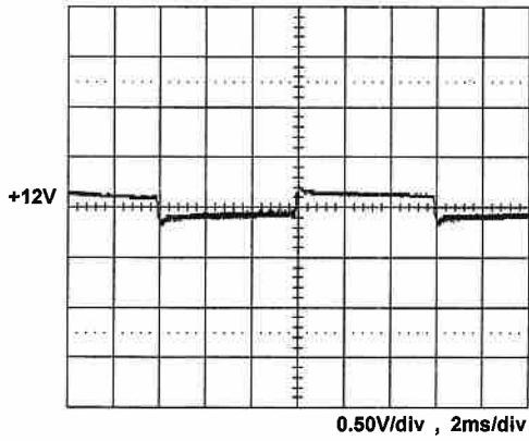
+12V step from 3.32A to 16.6A
