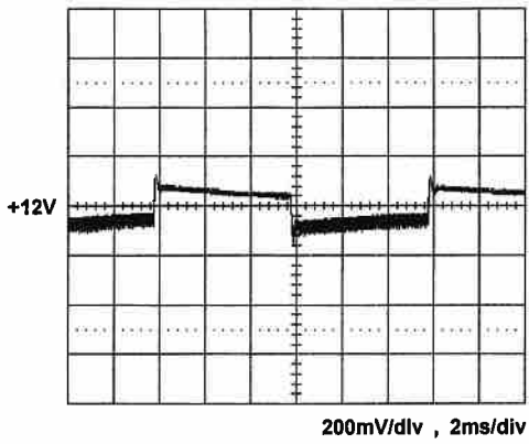
+12V step from 5A to 25A
