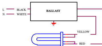
I5. one lamp
