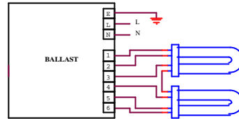
D. two lamp in series(for plastic case)
