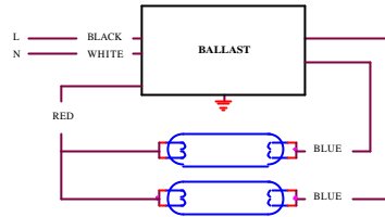
I2. two lamps in parallel
