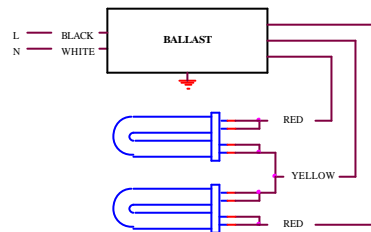
I6. two lamps in parallel
