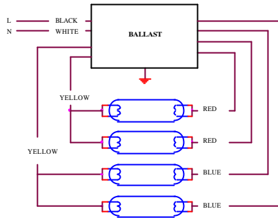
I4. four lamps in parallel
