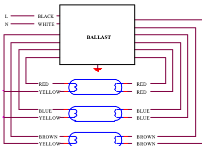
G. three lamps in parallel
