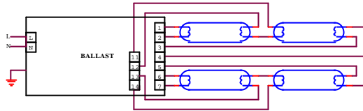
H. four lamp two in series & two parallel
