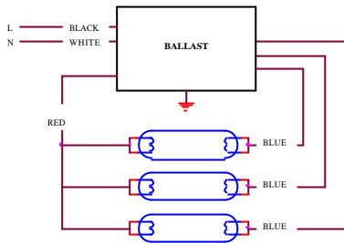
I3. three lamps in parallel
