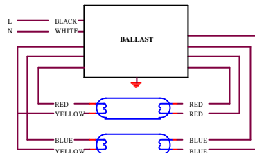
J. two lamps parallel
