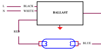
I1. one lamp
