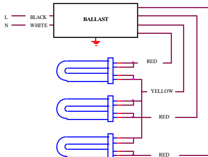
I7. three lamps in parallel
