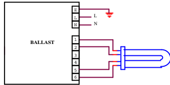
C. one lamp(for plastic case)
