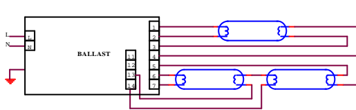
G. three lamp two in series & one parallel
