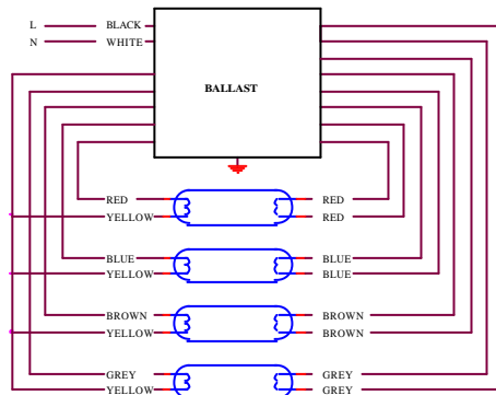
H. four lamps in parallel
