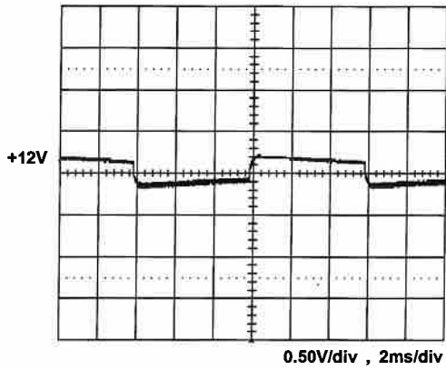
+12V step from 2.5A to 12.5A
