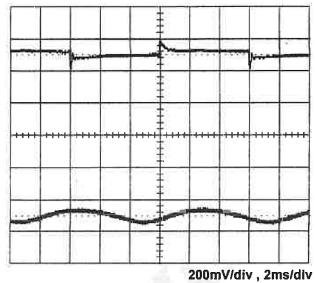
+5Vsb step from 0.2A to 1A +24V/9.996A
