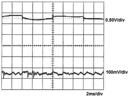
+24V step from 3.33A to 16.67A +5Vsb / 0.6A
